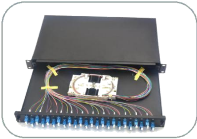
Model: SDPPD 1U-4U 6C-192C Available Material: Metal
