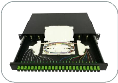
Model: SDPPDS 1U-4U 6C-192C Available Material: Metal
